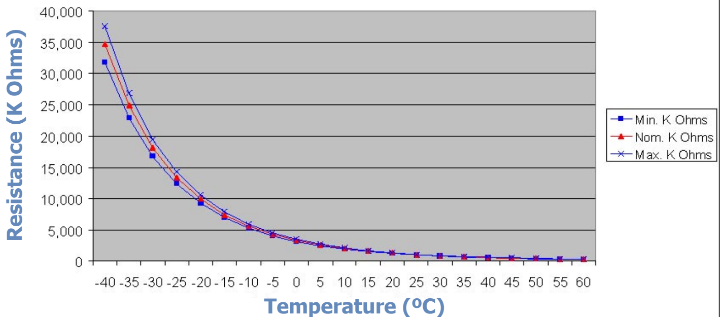
Resistance Characteristic Curve
